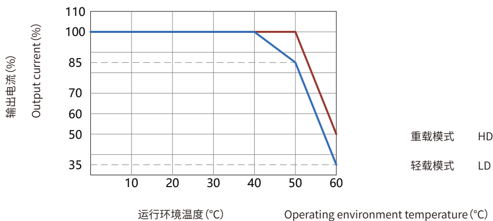
Capacity reduction data & Environment temperature
