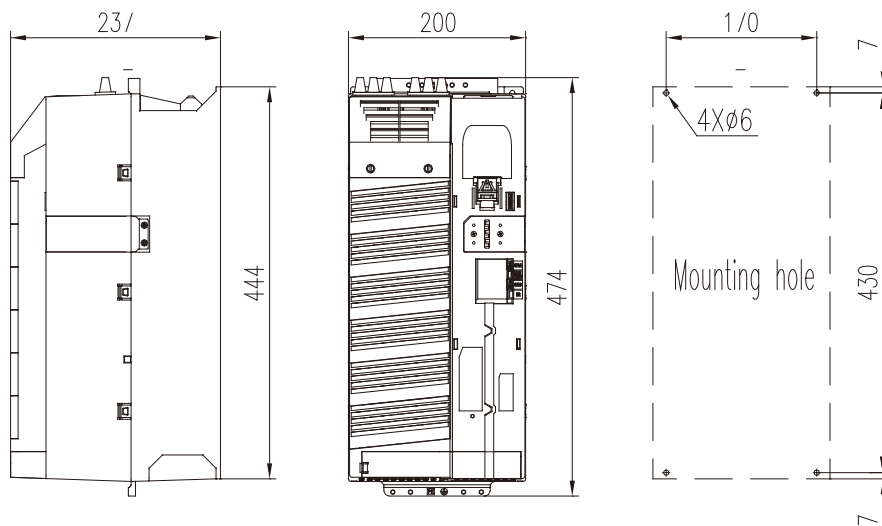
PM25 Power Module B3's dimensions (Unit:mm) Fixing requires 4 M5 combination screws, 4 M5 nuts, tightening torque: 4Nm Ventilation space at the top and bottom: 100mm, no need on the side. After installing the control module, the installation depth increases accordingly.
