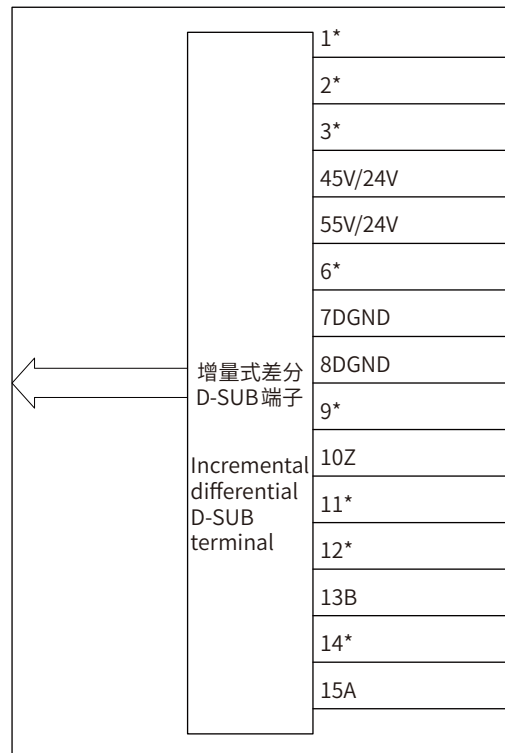
编码器接口 (CM25-XX- PE, 单端) Encoder interface (CM25-XX-PE, single-ended)
