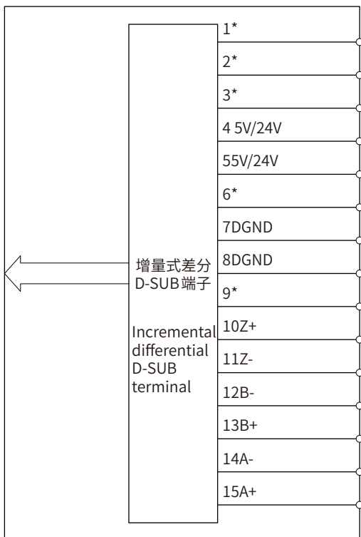
编码器接口 (CM25-XX-P E, 差分) Encoder interface (CM25-XX-PE, differential)
