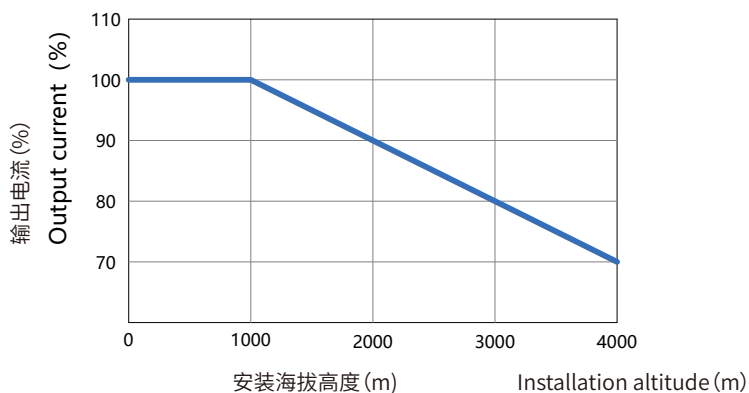
Capacity reduction data & Installation altitude
