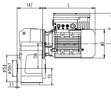
F205FC/F305FC
