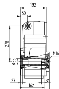
F207SK/F307SK F207AK/F307AK
