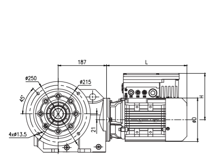
Flange-mounted F
