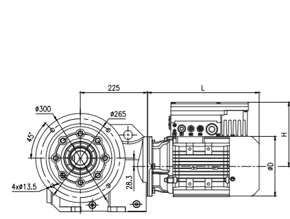
Flange-mounted F
