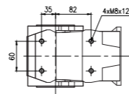
Shaft-mounted A
