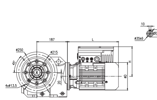
Flange-mounted F
