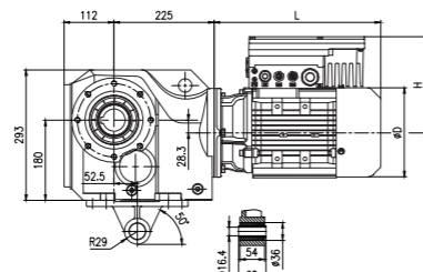
Torque arm-mounted with accessory T
