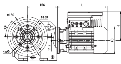
Flange-mounted F
