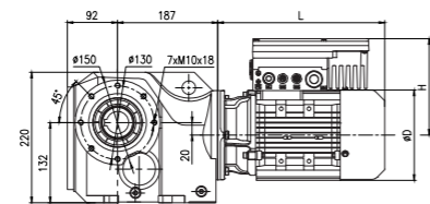
Short flange-mounted S
