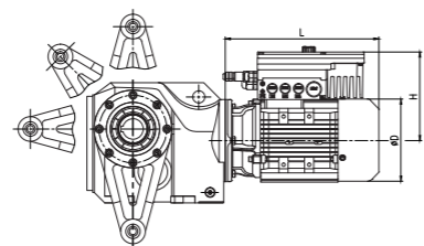
Torque arm-mounted with side accessory M
