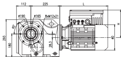
Short flange-mounted S
